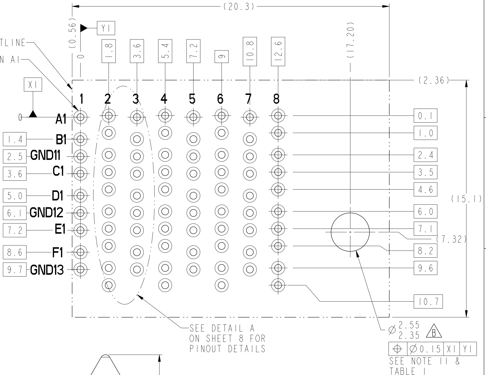
BP HOLE PATTERN COMPONENT SIDE RIGHT POLARIZING / GUIDE MODULE BACKPLANE FOOTPRINT
