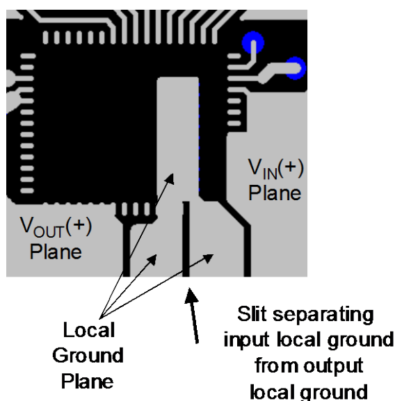
Figure 8. Layout of power and ground planes.
