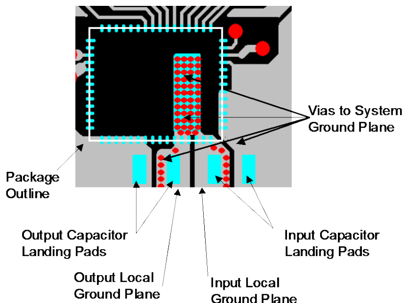
Figure 9. Use of vias connecting local and system ground.
