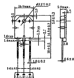
(TO-3P)
