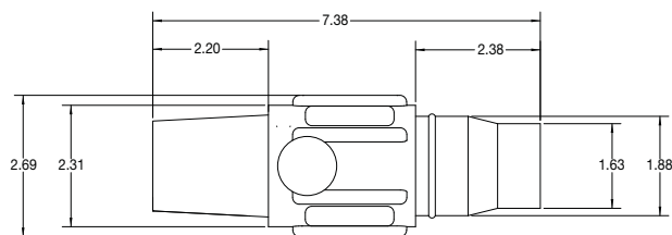
FEMALE CONNECTOR
