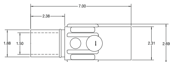
MALE CONNECTOR
