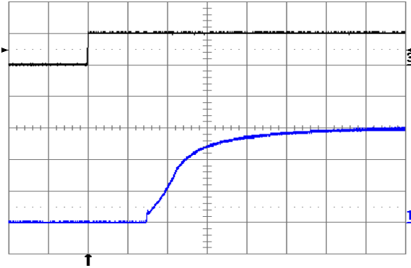
Fig. 6.0V.9: Turn-on transient at full rated load current (resistive) with no output capacitor at V_{in} = 24V , triggered via ON/OFF pin. Top trace: ON/OFF signal (5 V/div.). Bottom trace: output voltage (2 V/div.). Time scale: 1 ms/div.
