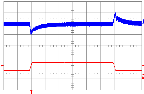
Fig. 1.5V.11: Output voltage response to load current step-change (3.75 A – 7.5 A – 3.75 A) at V_{in} = 24V . Top trace: output voltage (100 mV/div.). Bottom trace: load current (5 A/div.). Current slew rate: 0.1 A/ \mu s . C_o = 1 \mu F ceramic. Time scale: 0.2 ms/div.
