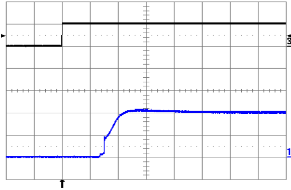
Fig. 1.0V.9: Turn-on transient at full rated load current (resistive) with no output capacitor at V_{in} = 24V , triggered via ON/OFF pin. Top trace: ON/OFF signal (5 V/div.). Bottom trace: output voltage (0.5 V/div.). Time scale: 1 ms/div.
