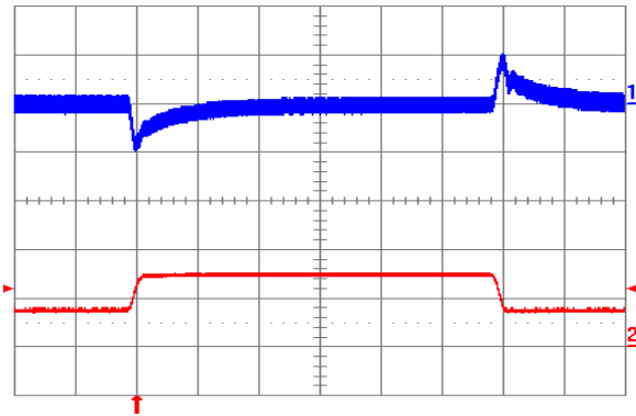
Fig. 1.0V.11: Output voltage response to load current step-change (3.75 A – 7.5 A – 3.75 A) at V_{in} = 24V . Top trace: output voltage (100 mV/div.). Bottom trace: load current (5 A/div.). Current slew rate: 0.1 A/µs. C_o = 1 \mu F ceramic. Time scale: 0.2 ms/div.
