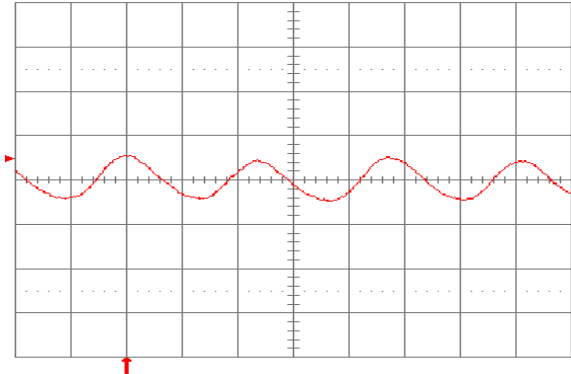
Fig. 3.3V.15: Input reflected ripple current, i_c (100 mA/div.), measured at input terminals at full rated load current and V_{in} = 24\ \text{V} . Refer to Fig. 3.3V.14 for test setup. Time scale: 1\ \mu\text{s}/\text{div} .
