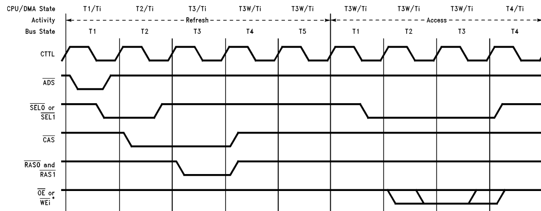
FIGURE 3-11. Zones 0, 1 Access Delayed by a Refresh Transaction (No Wait)
