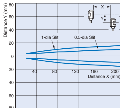
E3T-FT1□ + E39-S64 Slit (Order Separately)(Enlarged graph)
