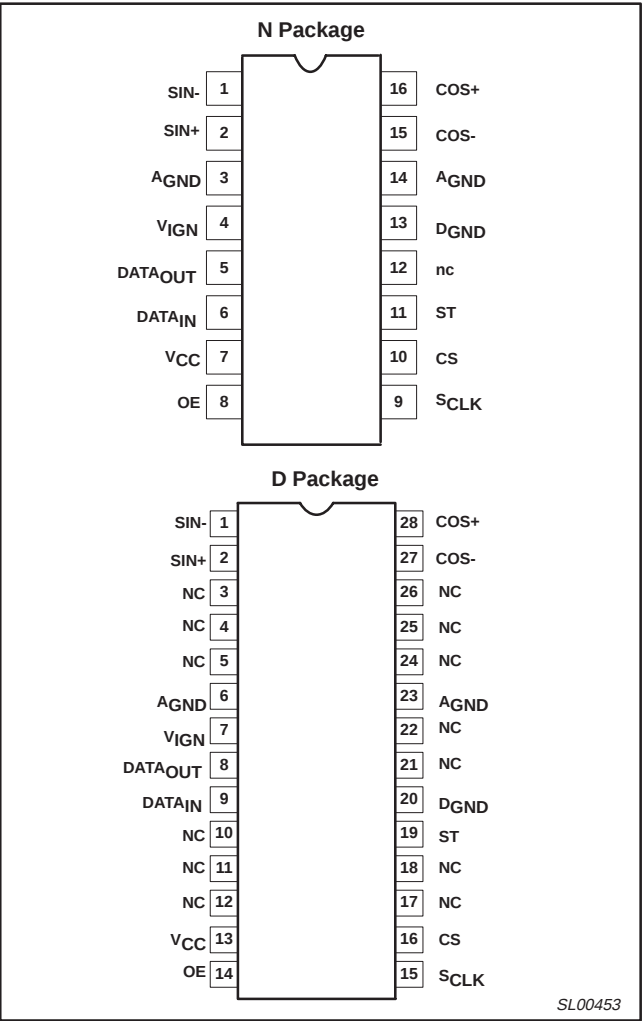
Figure 1. Pin configuration
