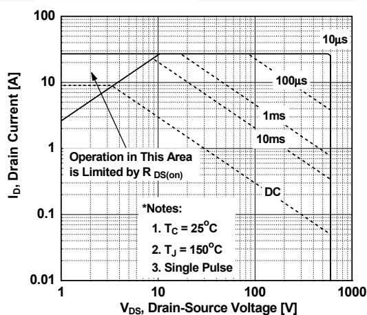
Figure 10. Maximum Safe Operating Area for FCPF9N60NT
