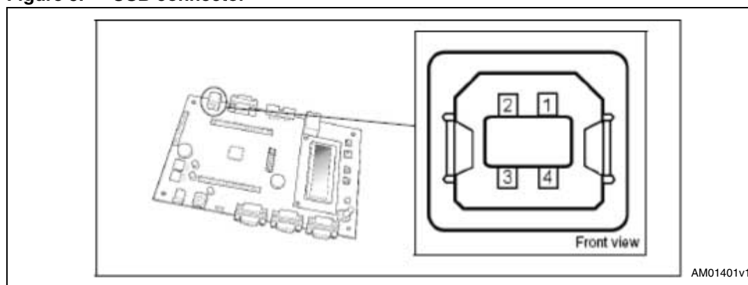
Figure 5. USB connector
