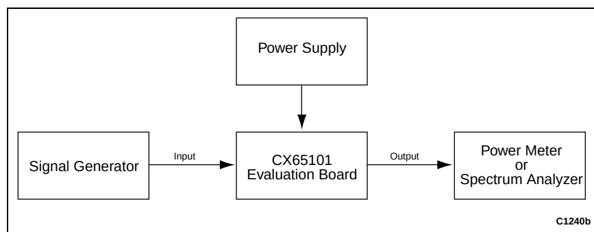
Figure 12. CX65101 Evaluation Board Testing Configuration
