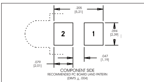
COMPONENT SIDE RECOMMENDED PC BOARD LAND PATTERN (DIM'S \pm .004 \pm 0.1\text{MM} )
