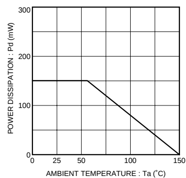
Fig.3 Derating curve
