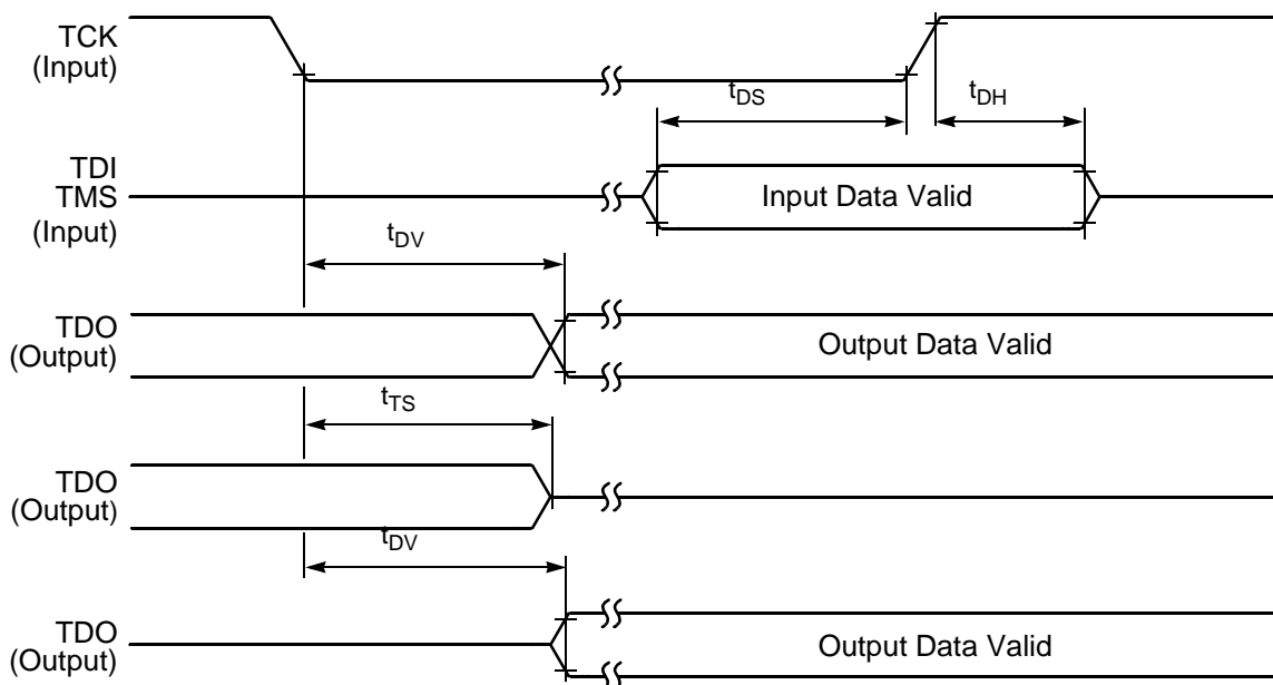
Figure 16. Test Clock Input Timing Diagram
