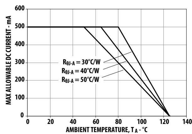
Figure 13 Maximum Forward Current vs. Ambient Temperature. Derated based on T_{JMAX} = 125^{\circ}C , R_{\theta J-A} = 30^{\circ}C/W , 40^{\circ}C/W , and 50^{\circ}C/W .
