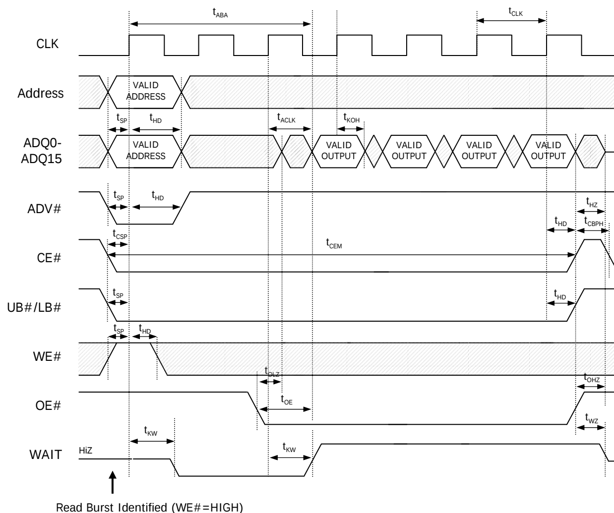
Figure 2. Synchronous Read Access Timing
