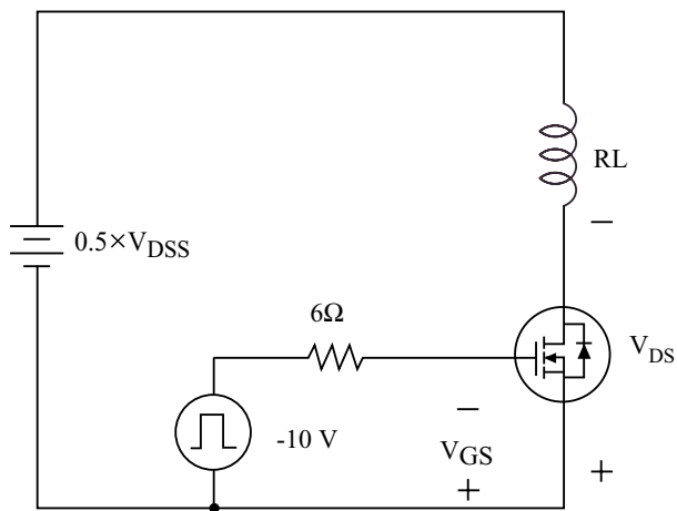
Fig10. Resistive Load Switching
