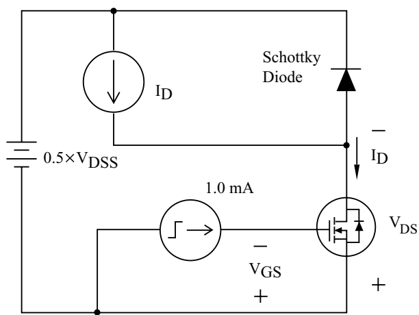
Fig9. Gate Charge Circuit and Wave Form
