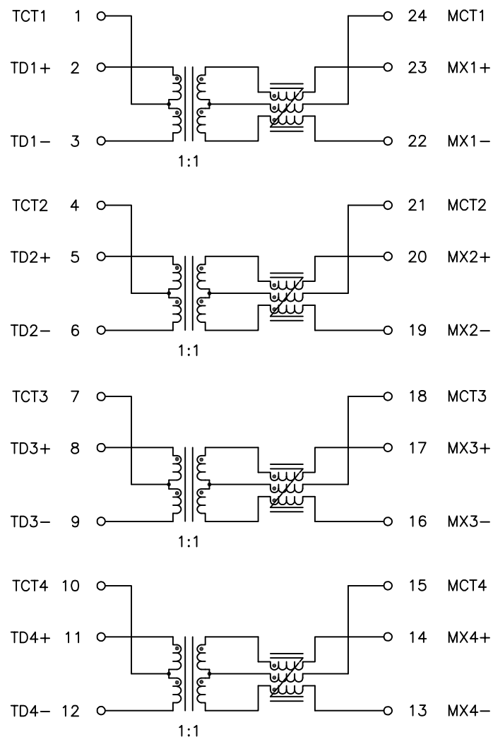
SCHEMATIC
