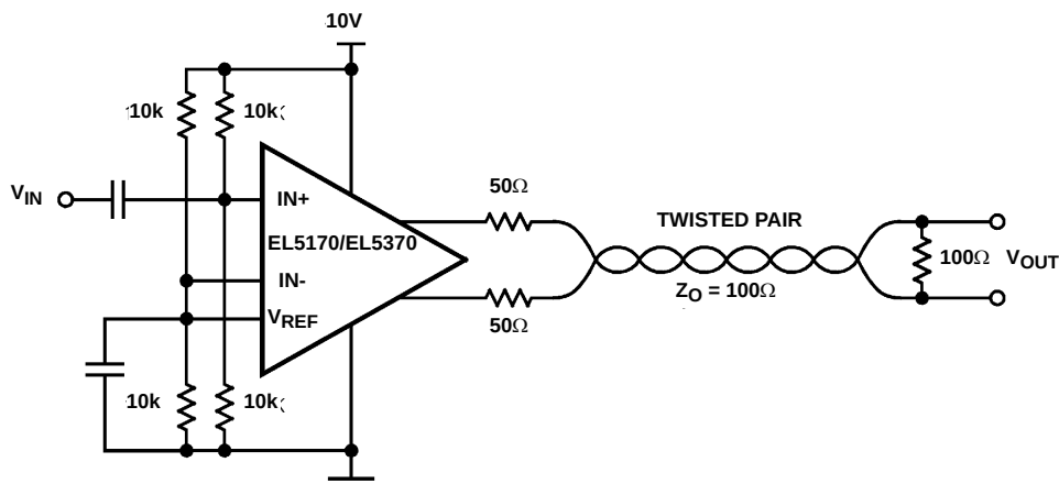
FIGURE 22. SINGLE SUPPLY TWISTED PAIR DRIVER
