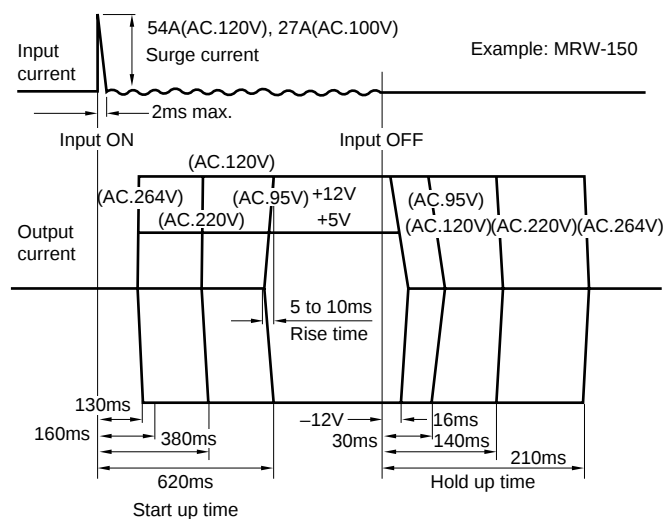
SURGE CURRENT, START UP TIME AND HOLD UP TIME TEMPERATURE: 25°C
