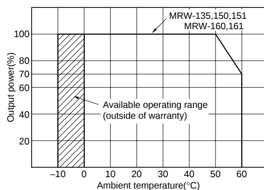
OUTPUT POWER-AMBIENT TEMPERATURE(DERATINGS)
