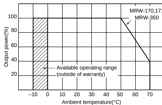
OUTPUT POWER-AMBIENT TEMPERATURE(DERATINGS)
