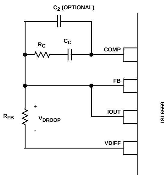
FIGURE 12. COMPENSATION CONFIGURATION FOR LOAD-LINE REGULATED ISL6559 CIRCUIT
