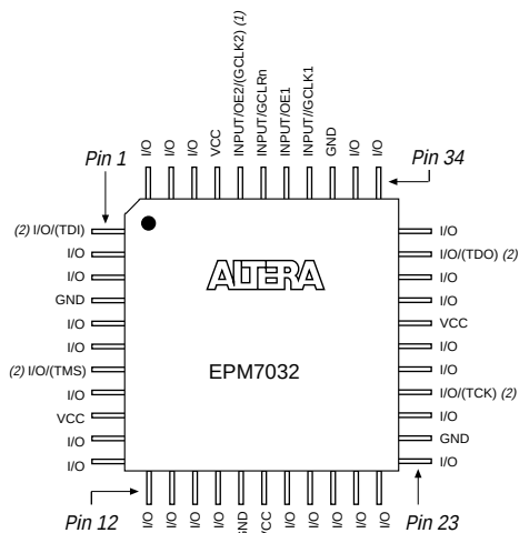
44-Pin PQFP
