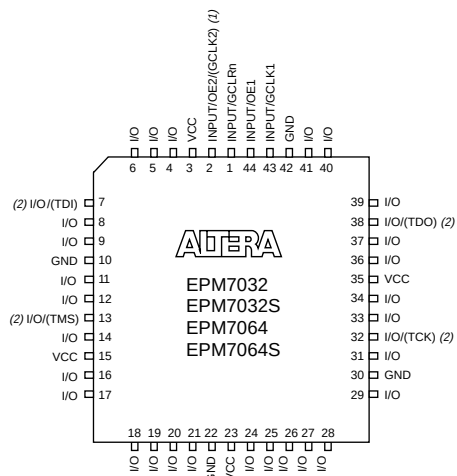
44-Pin PLCC
