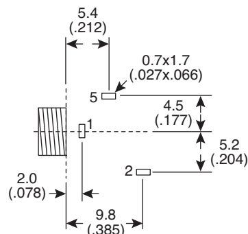
PCB Hole Layout (Bottom View)
