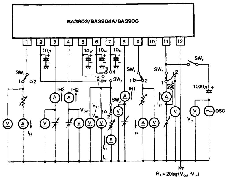
Figure 1 Test circuit
