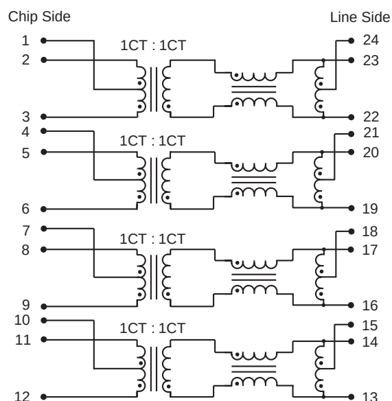
S558-5999-P3 S558-5999-T3
