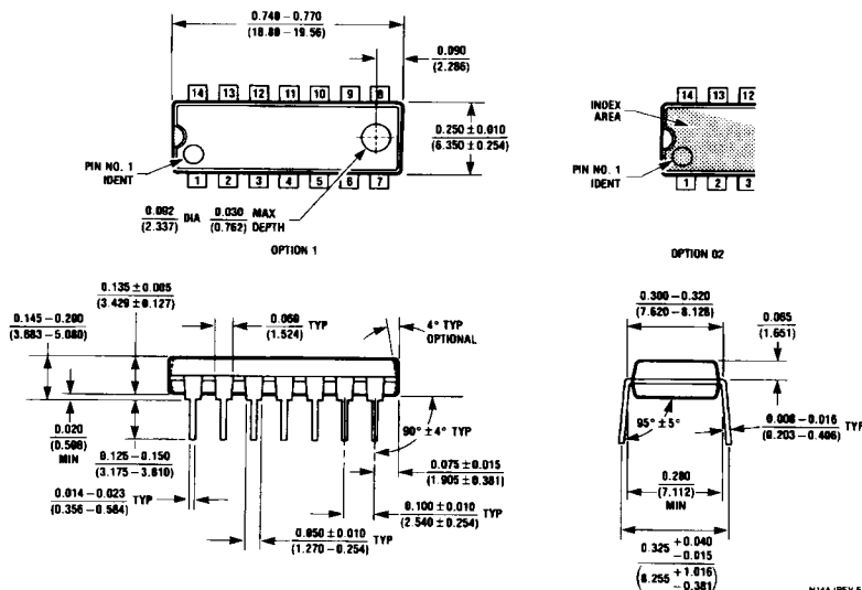
Molded Dual-In-Line Package (N) Order Number CD4070BCN or CD4077BCN NS Package Number N14A
