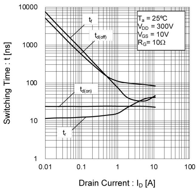
Fig.19 Switching Characteristics
