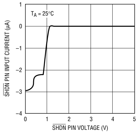
\overline{SHDN} Pin Input Current vs Voltage
