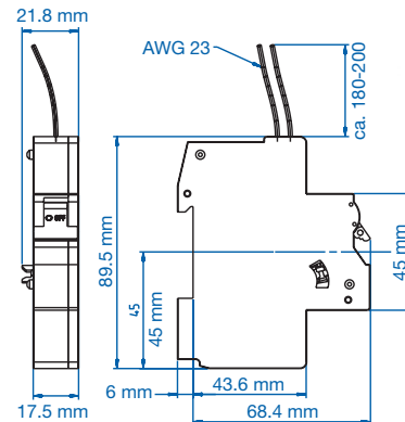
Dimensions UA120UM.
