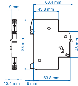
Dimensions HLS11M.
