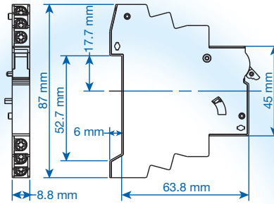
Dimensions HxxUM.
