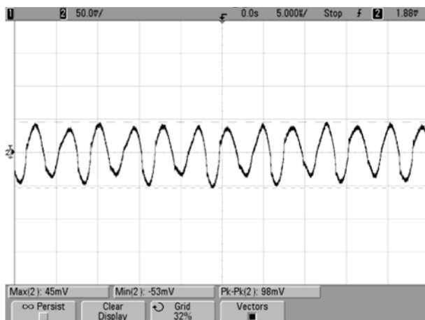
Output Ripple and Noise (Vin=75V, Iout=0A, Load=0, Ta=+25°C., ScopeBW=20MHz)
