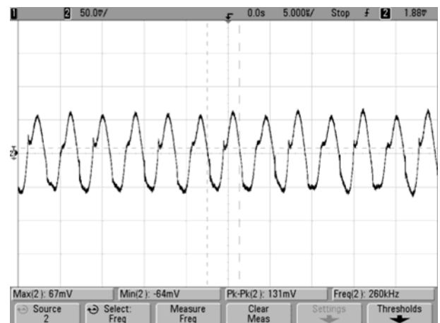
Output Ripple and Noise (Vin=75V, Iout=25A, Load=0, Ta=+25°C., ScopeBW=20MHz)
