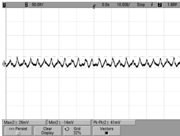
Output Ripple and Noise (Vin=48V, Iout=0A, Load=0, Ta=+25°C., ScopeBW=20MHz)
