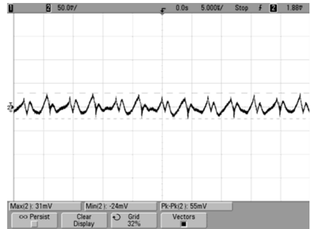
Output Ripple and Noise (Vin=48V, Iout=25A, Load=0, Ta=+25°C., ScopeBW=20MHz)
