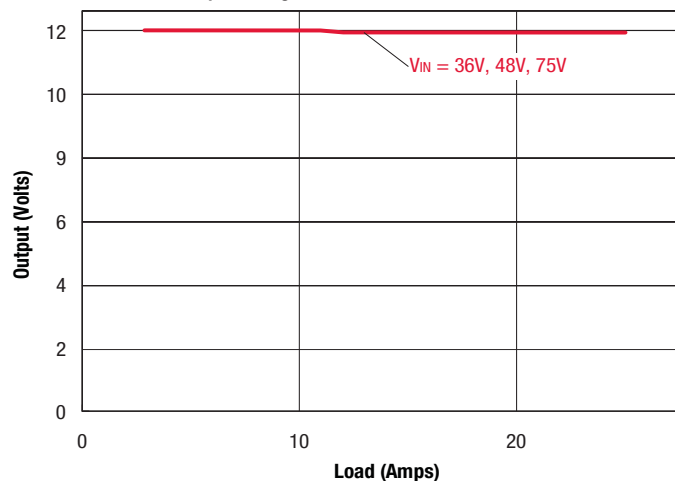
Output Voltage vs Load Current at -40°C.
