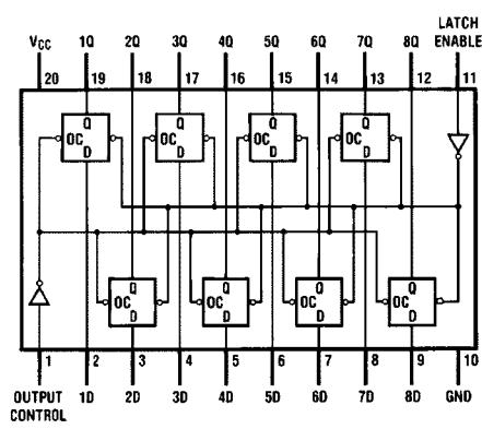
Top View MM74HCT573
