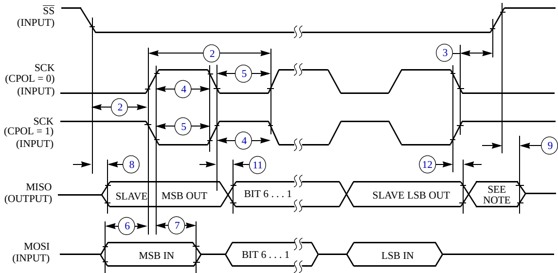
NOTE: 1. Not defined, but normally MSB of character just received Figure 17. SPI Slave Timing (CPHA = 0)
