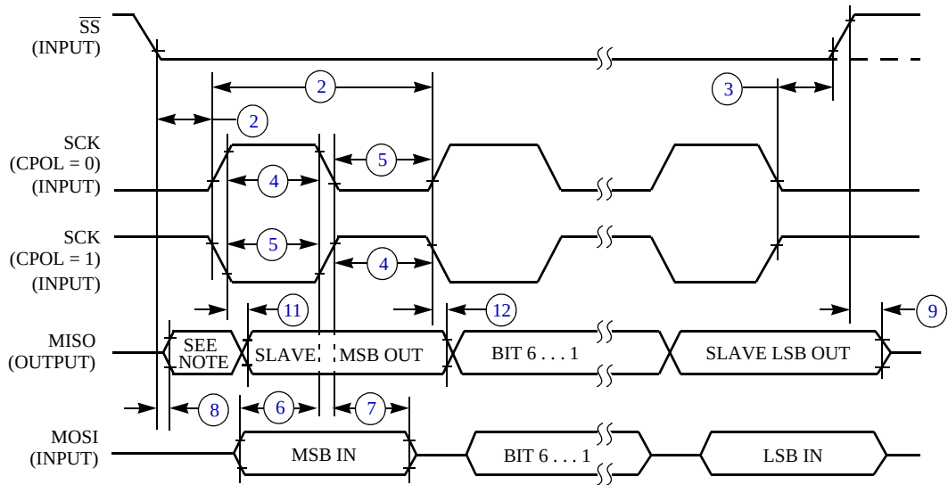
NOTE: 1. Not defined, but normally LSB of character just received Figure 18. SPI Slave Timing (CPHA = 1)
