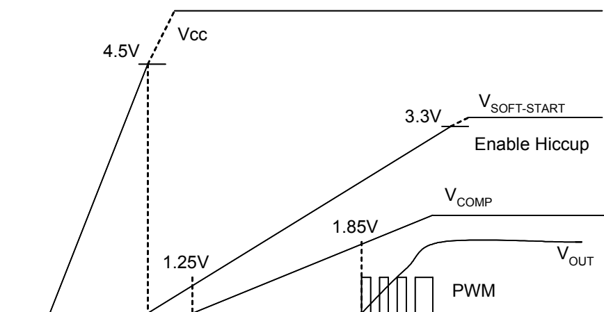
Figure 6a. SC2441A Start-up Timing Diagram
