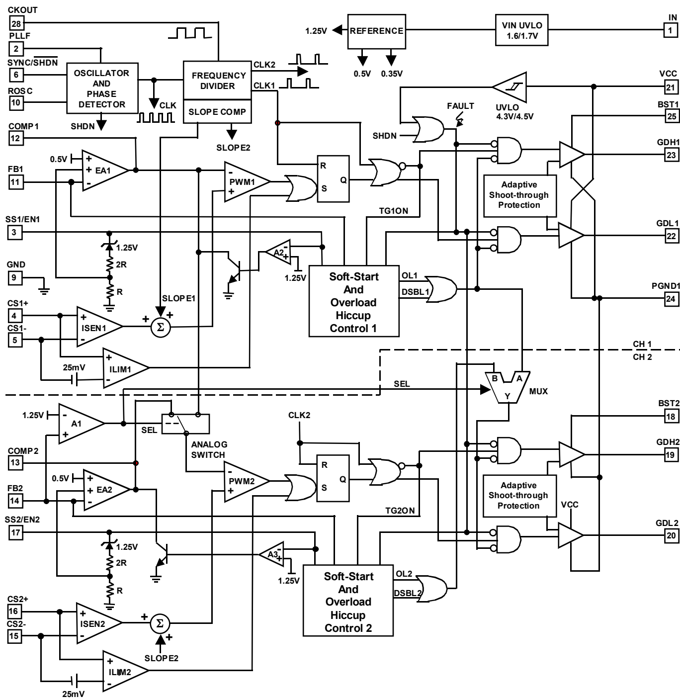
Figure 2 Functional Diagram of the Step-down Controllers
