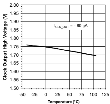
Clock Output High Voltage vs Temperature
