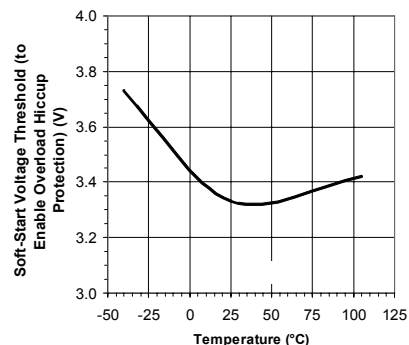
Soft-Start Voltage Threshold (to Enable Overload Hiccup Protection) vs Temperature
