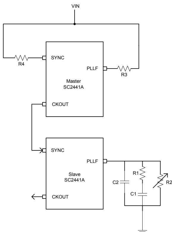
Figure 15. Master-Slave Synchronization
