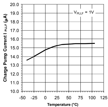
Charge Pump Current I_{PLL} vs Temperature
