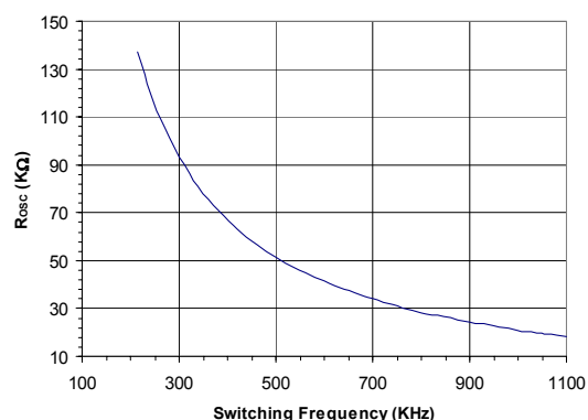
R_{OSC} vs. Step-down Channel Switching Frequency
