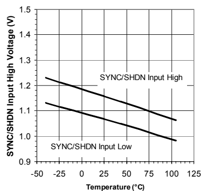
SYNC/SHDN Input Voltage vs Temperature
