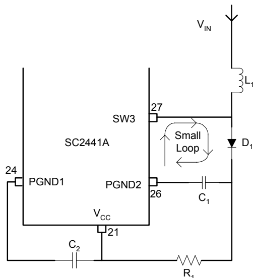
Figure 9. Step-Up Section Layout Illustration
