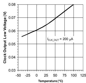
Clock Output Low Voltage vs Temperature
