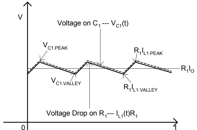
Figure 13. Voltage Waveform C_1 and R_1
