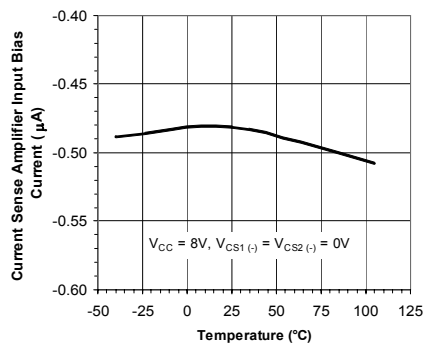
Current Sense Amplifier Input Bias Current vs Temperature (Non-inverting Pin)
