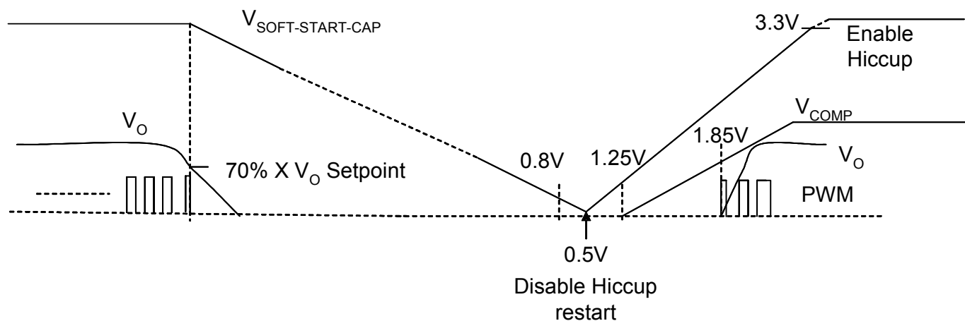
Figure 6b. SC2441A Overload Hiccup Operation Timing Diagram
