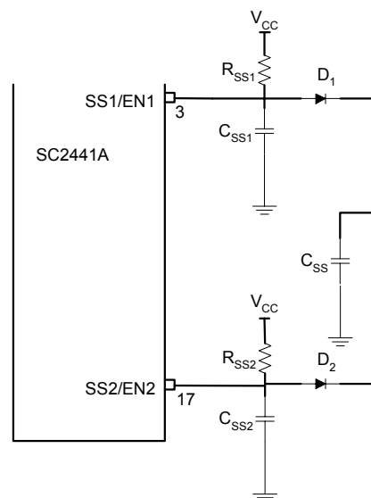
Figure 11. Coincident Soft-Start for Step-Down Converters
