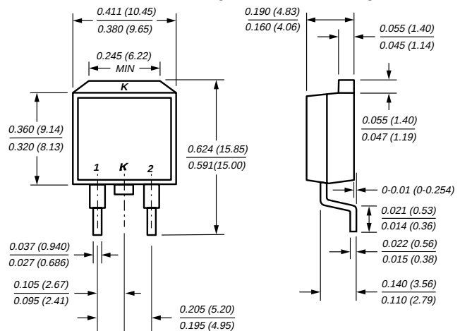
TO-263AB (FEPB6AT Series)
