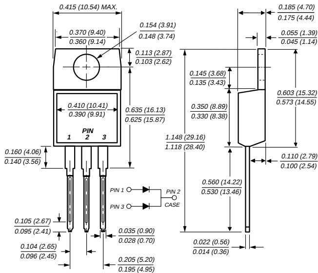
TO-220AB (FEP6AT Series)
