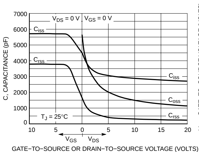
Figure 7. Capacitance Variation
