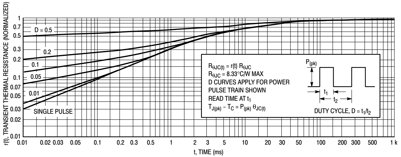
Figure 10. Thermal Response
