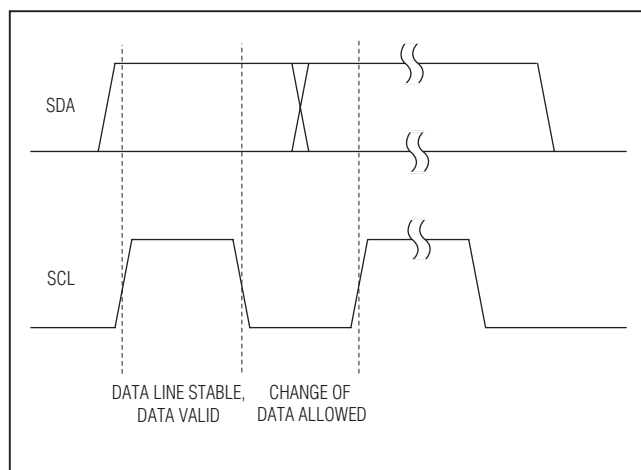
Figure 9. Bit Transfer
