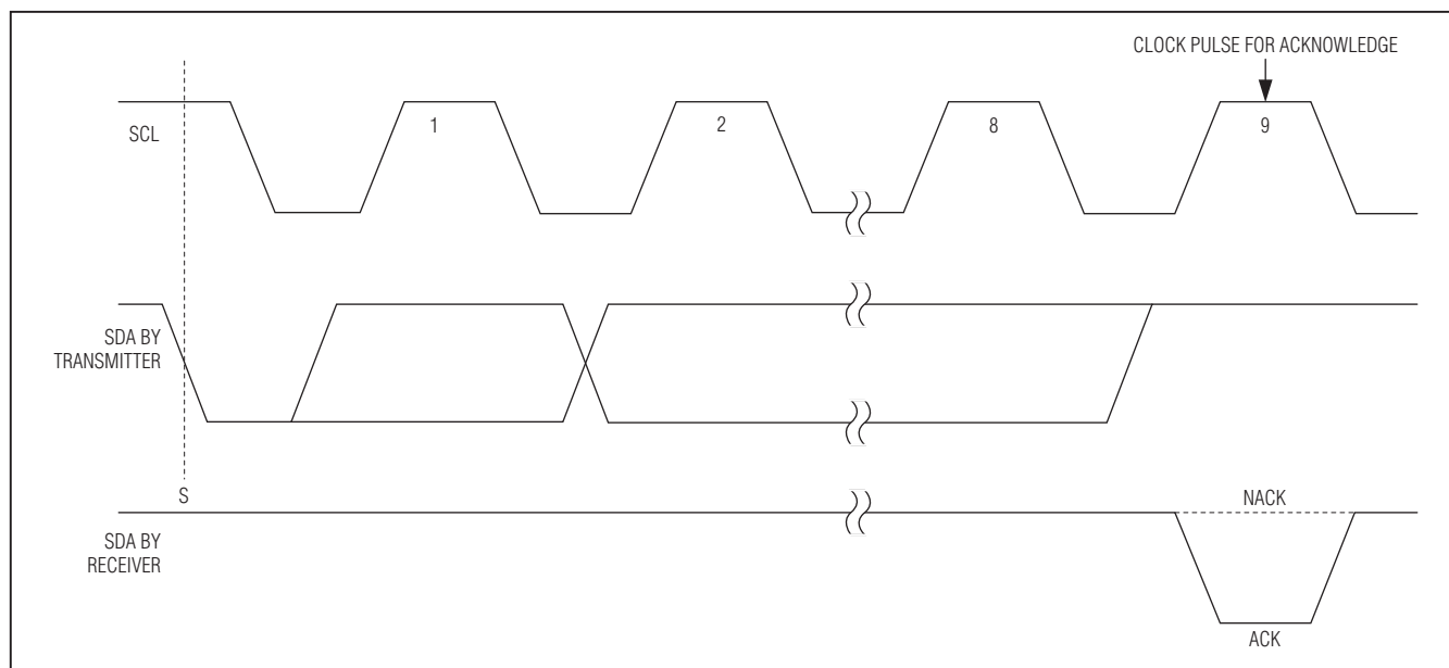
Figure 11. Acknowledge
