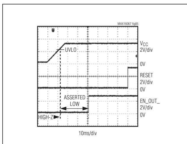
Figure 5. RESET and EN_OUT_ During Power-Up, EN_OUT_ is in Push-Pull Active-High Configuration
