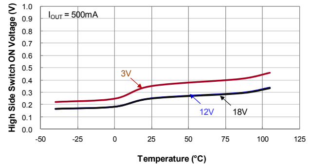
HighSide Switch On Voltage ( V_{DD} - V_{OH} ) vs. Temperature
