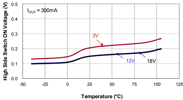
HighSide Switch On Voltage ( V_{DD} - V_{OH} ) vs. Temperature
