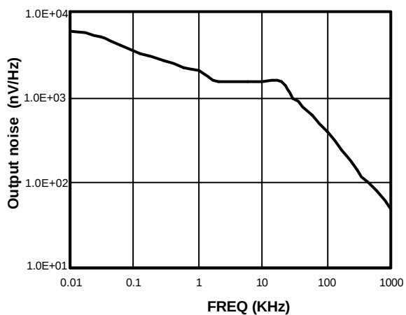
Output Noise Spectral Density vs. Frequency
