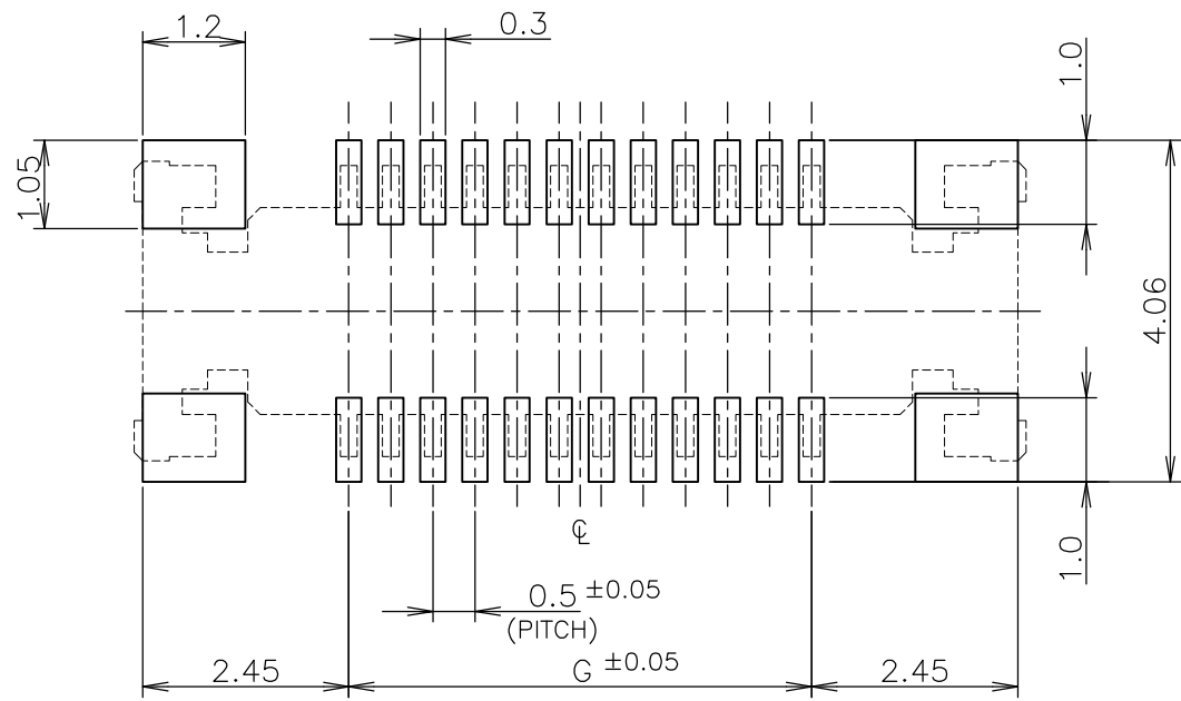
(T=0.6 MIN.) P.C. BOARD LAYOUT (REF.)
