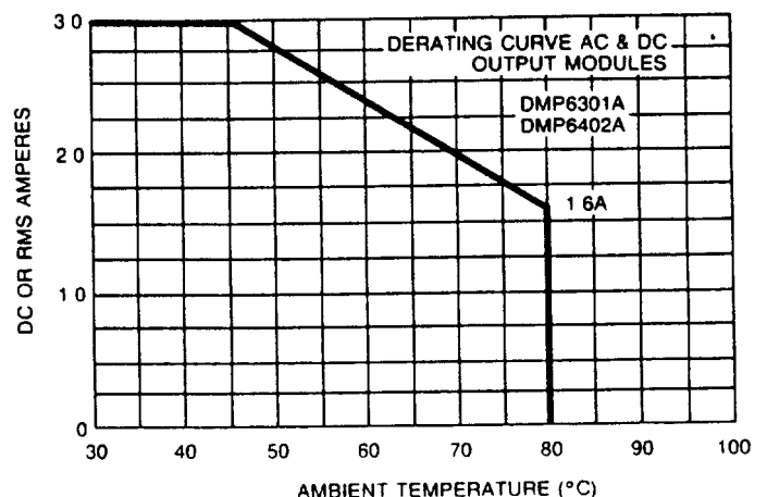
Figure 1. Maximum Output Current vs Ambient Temperature
