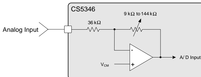
Figure 10. CS5346 PGA
