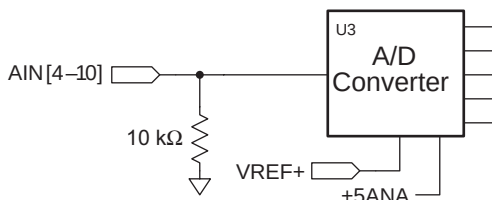
Figure 3-7. Schematic of XP8500 Unconditioned Inputs
