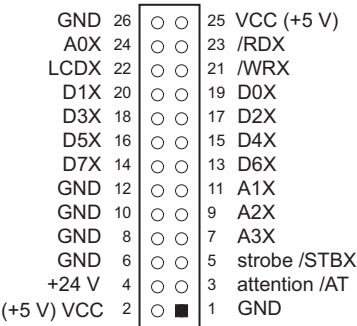
Figure A-1. PLCBus Pin Diagram
