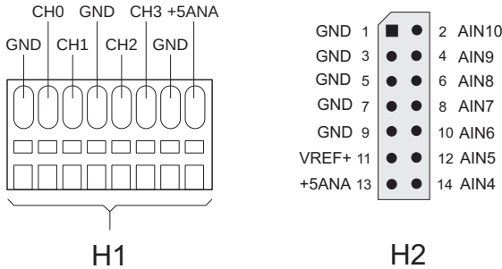
Figure 3-1. XP8500 Pin Assignments
