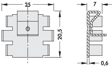
TO 220
