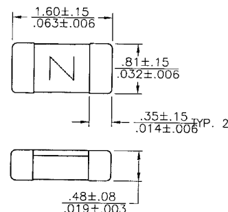
Dimensions mm/(inches) Drawing Not to Scale
