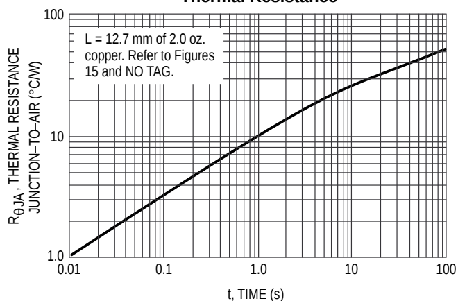
Figure 14. DW and P Suffix Transient Thermal Resistance
