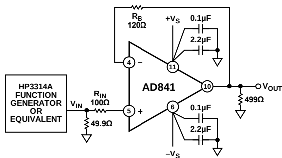
Figure 25. Unity-Gain Buffer Amplifier Configuration (PDIP Pinout)
