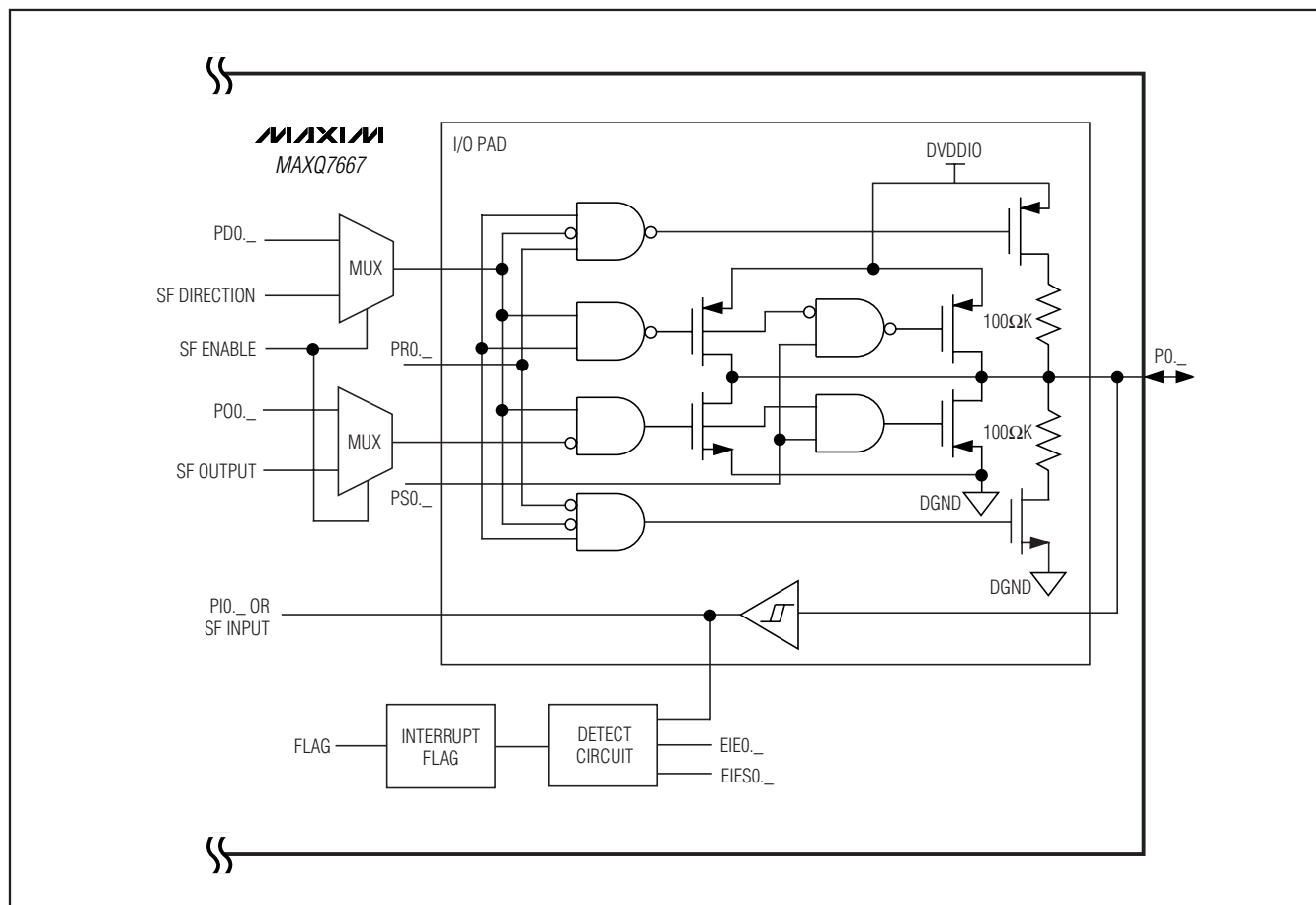
Figure 13. Port 0 Digital I/O Basic Circuitry. Port 1 Circuitry is the Same as Port 2.
