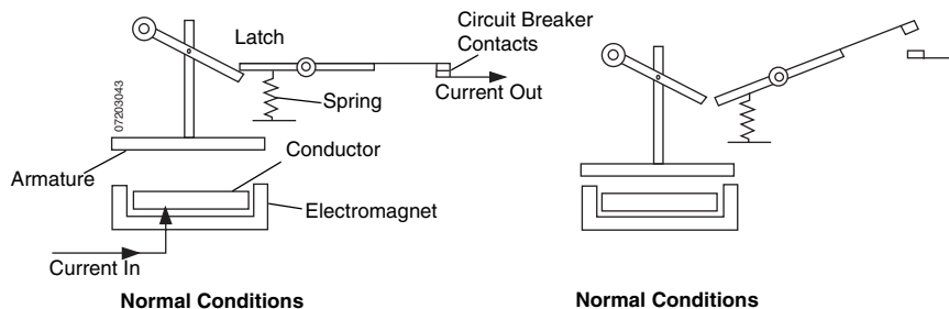
Figure 2: Magnetic Tripping
