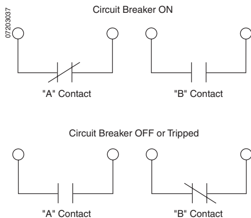
Figure 8: Alarm Switch Accessory
