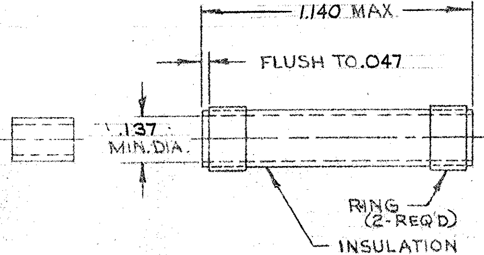
BUSHING
